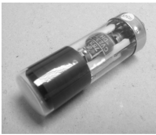
FIG. 1. A CV2302 28 mm cathode ray tube. Photo credit: langrex.co.uk.
